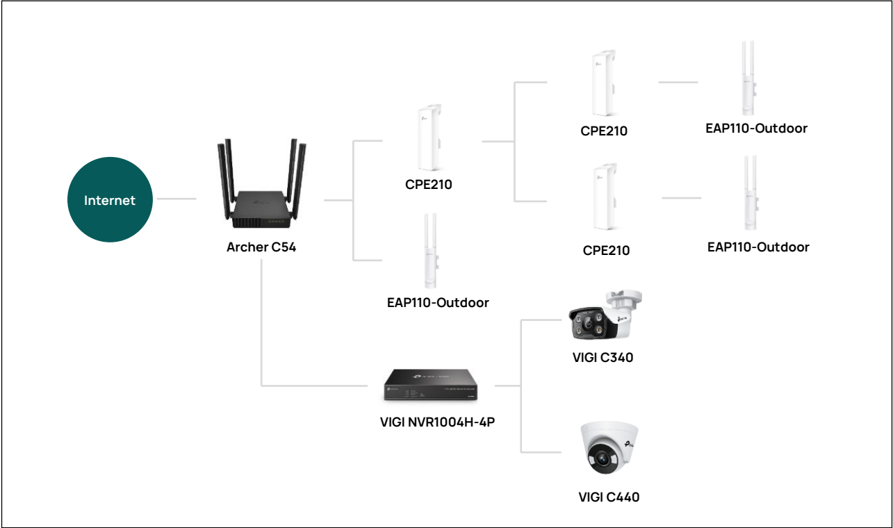
Topology
